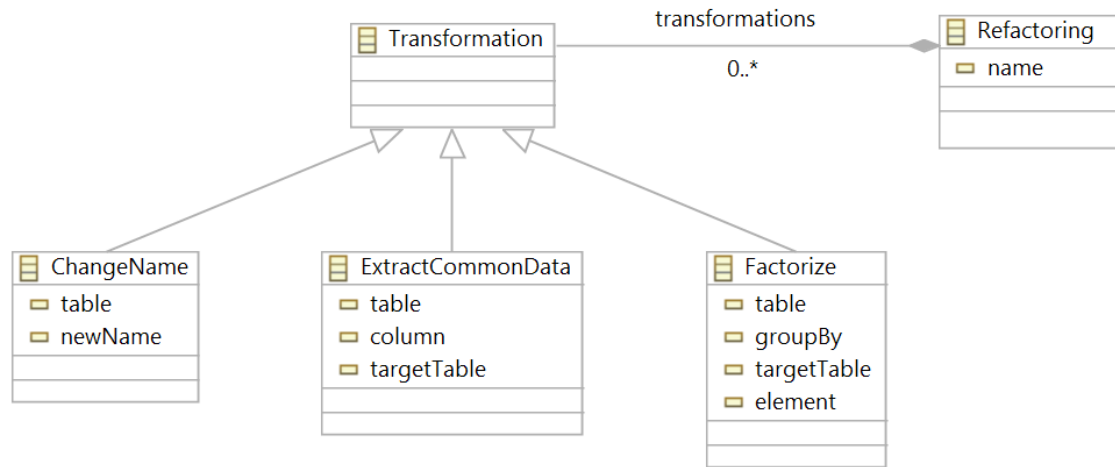
Figure 9. customized metamodel of the domain specific transformation language
